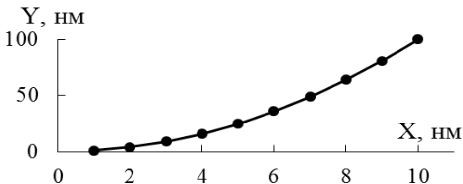
Figure 1. An example of the dependence of y on the parameter x
